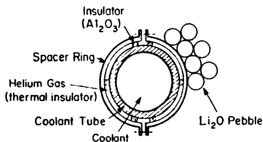
Figure 5: INTOR breeding blanket concept [6].
