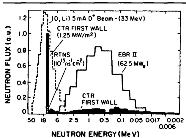
Figure 1: Typical neutron spectra for various nuclear facilities [3].
