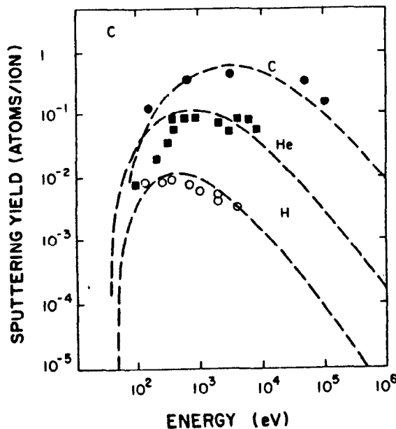
Figure 6a: Sputtering of carbon by H, He, C ions [7].
