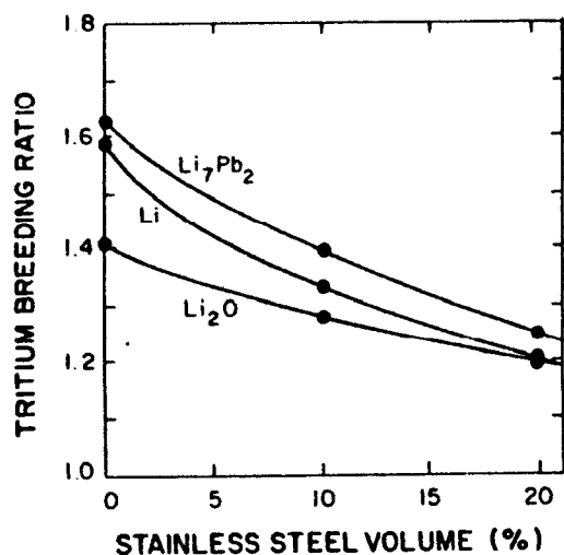
Figure 4: Attainable breeding ratio vs volume per cent stainless steel structure [2].
