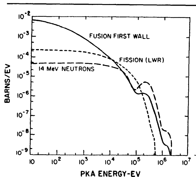
Figure 2: Primary knock-on spectra for copper in various nuclear facilities [3].
